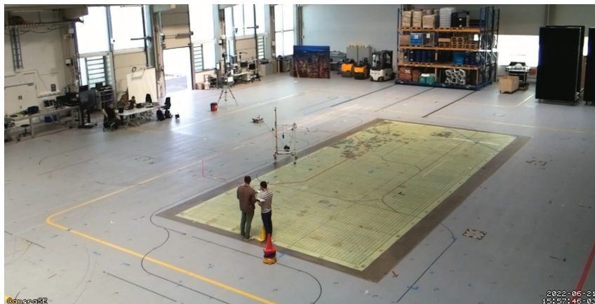
Figure 7.3: The measurement hall layout without absorber walls.
