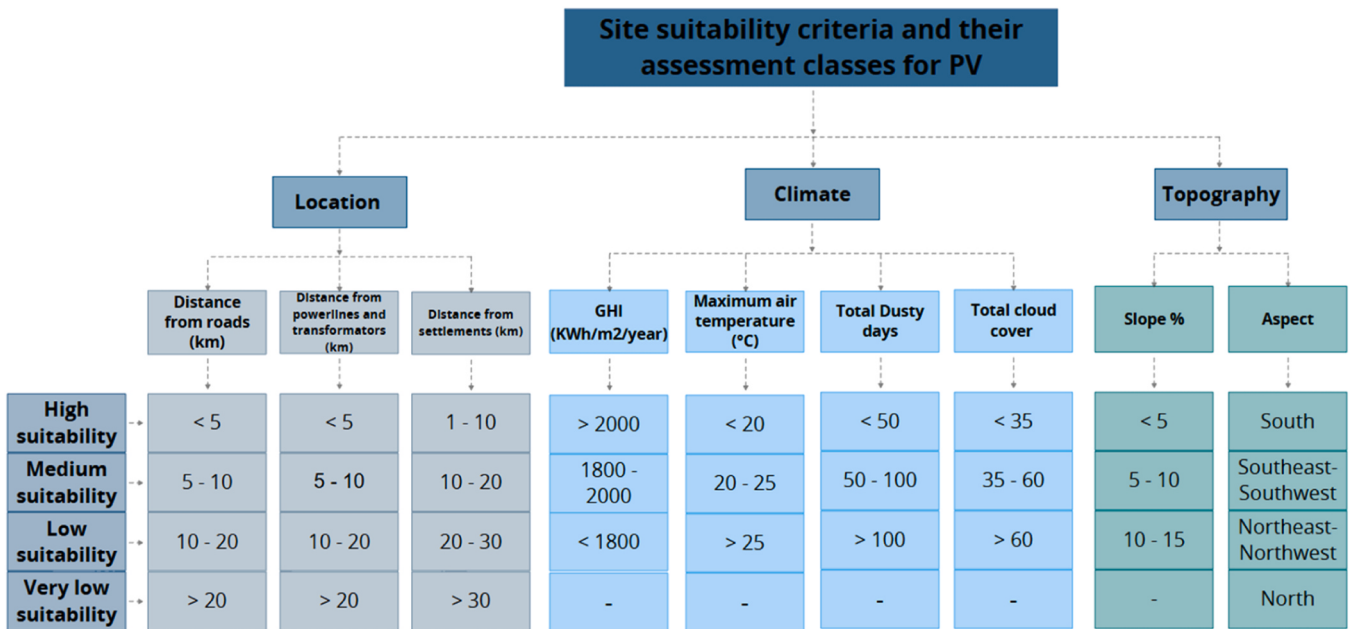
Fig. 2. Site suitability criteria and their assessment classes for PV parks.
