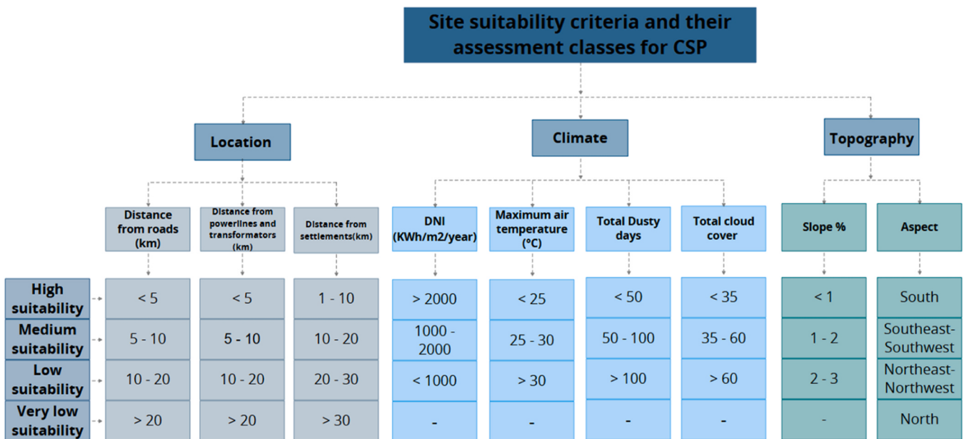
Fig. 3. Site suitability criteria and their assessment classes for CSP.
