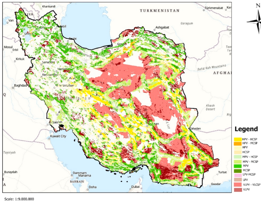
Fig. 5. Categorized suitable area for PV and CSP plant siting in Iran. Legend: VLPV: Very low suitability for PV, LPV: Low suitability for PV, MPV: Medium suitability for PV, HPV: High suitability for PV, VLCSP: Very low suitability for CSP, MCSP: Medium suitability for CSP, HCSP: High suitability for CSP.
